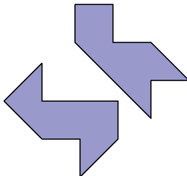
Figure 1: Identical sounding drums (taken from http://www.math.udel.edu/~driscoll/ )
